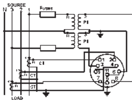
Fig. C2 Models 078-219 Wattmeter 3-phase 4-wire unbalanced load
