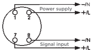
FIG. L MODELS 007-DI2, 007-DIA, 007-DIB, 007-DIC, 007-DIN, 007-DIT, 007-DIV, 007-DIW LED DIGITAL/ANALOG METER
