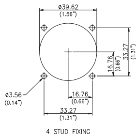
Model 362 surface mount cut-out
