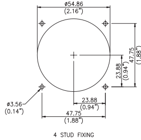
Model 363 surface mount cut-out
